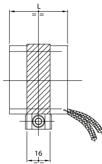
Nr.2 fascette da L 36 mm a L 60 mm No.2 bands from L 36 mm to L 60 mm
